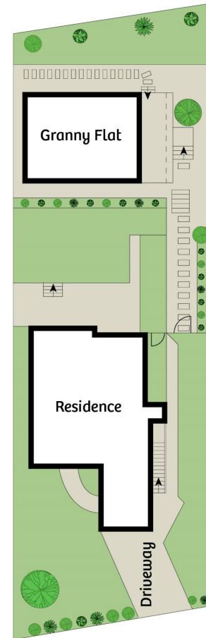
Site Plan
